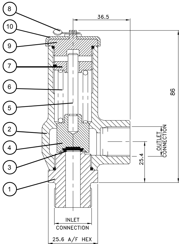
ILLUSTRATED SHOWING TYPE B BASIC SEALED WIRELOCK NO EASING GEAR
